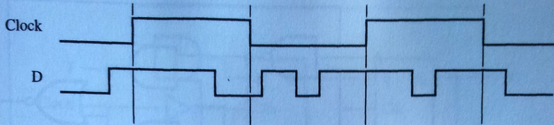
Figure P7.1 Timing diagram for problem 7.1.
